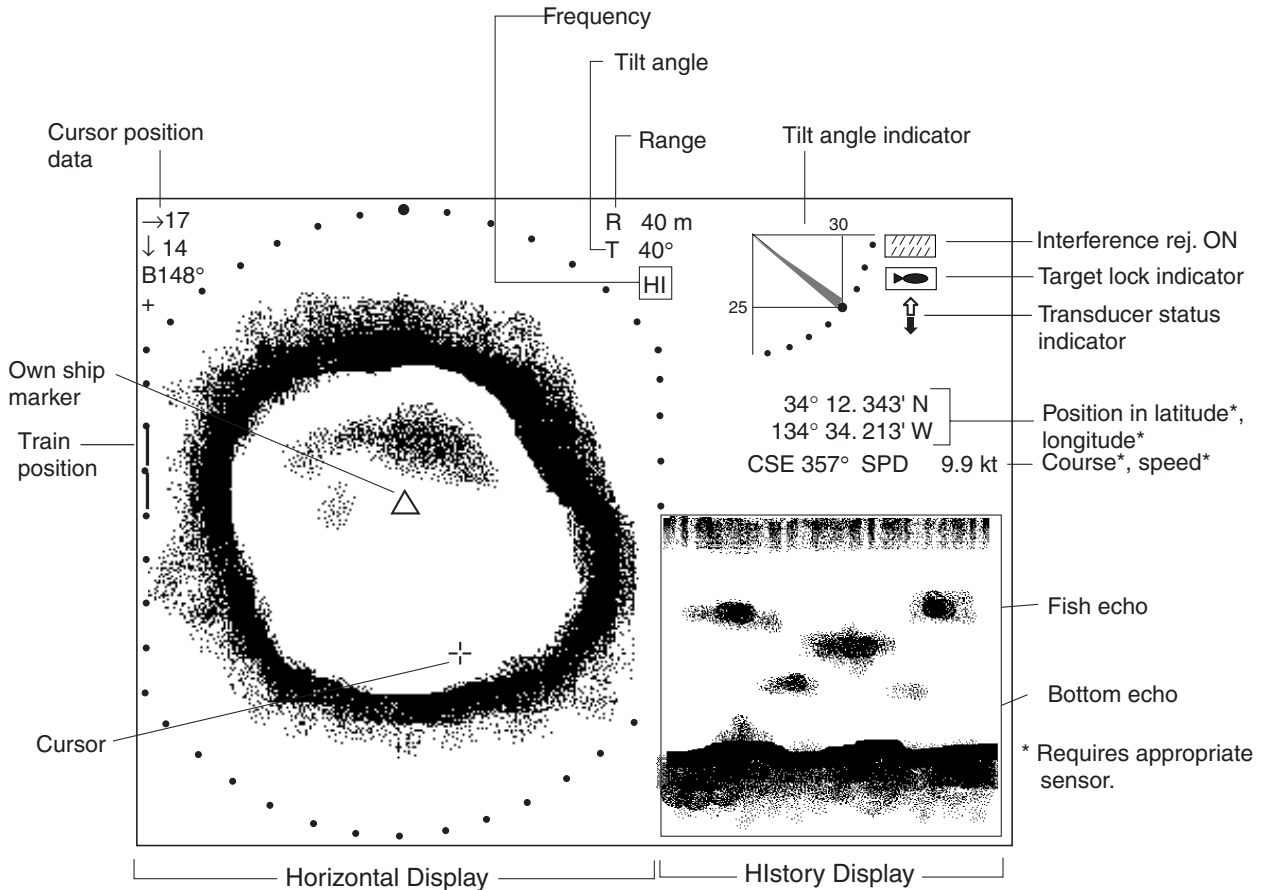
Horizontal/history display
