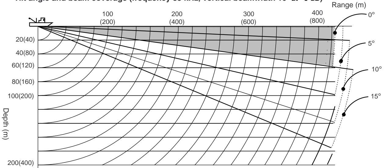
Vertical width of sonar beam
