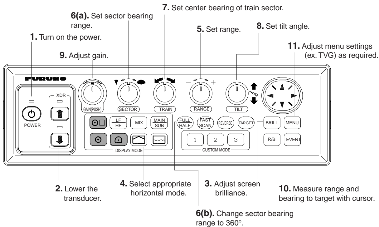
Control panel
