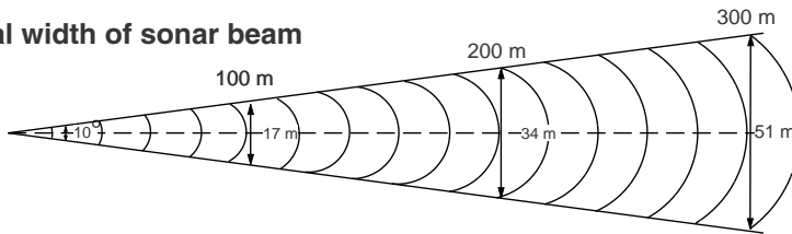
Tilt angle and beam coverage
