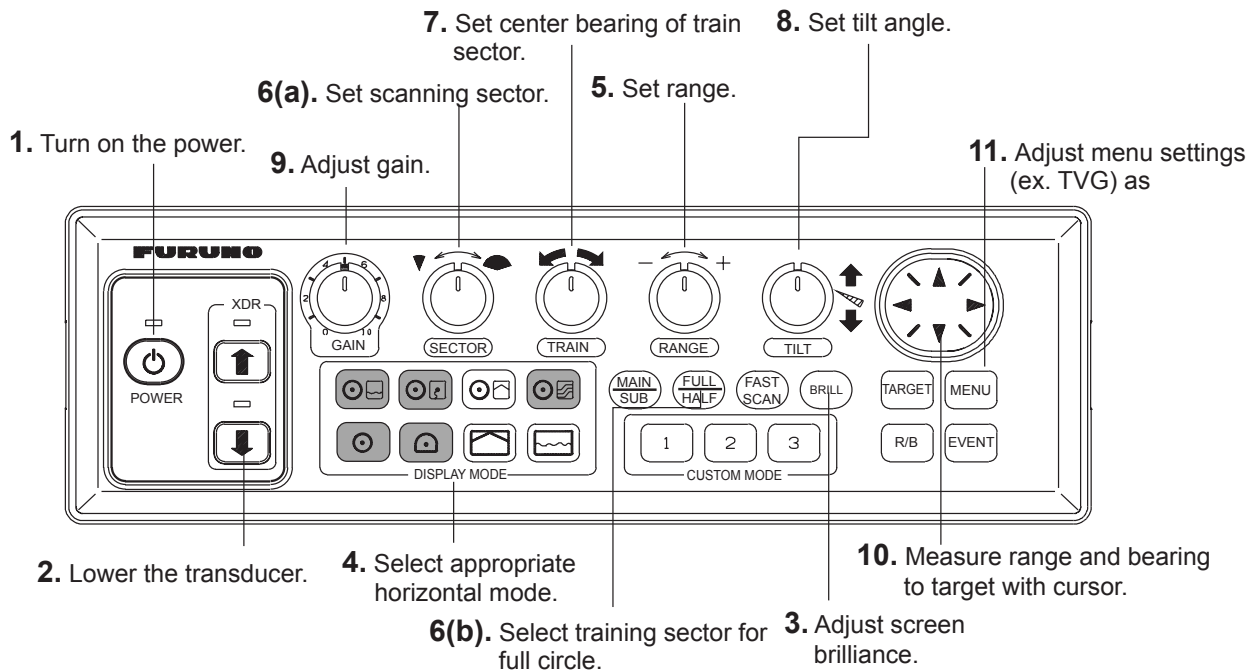
Figure 2-1 Control panel
