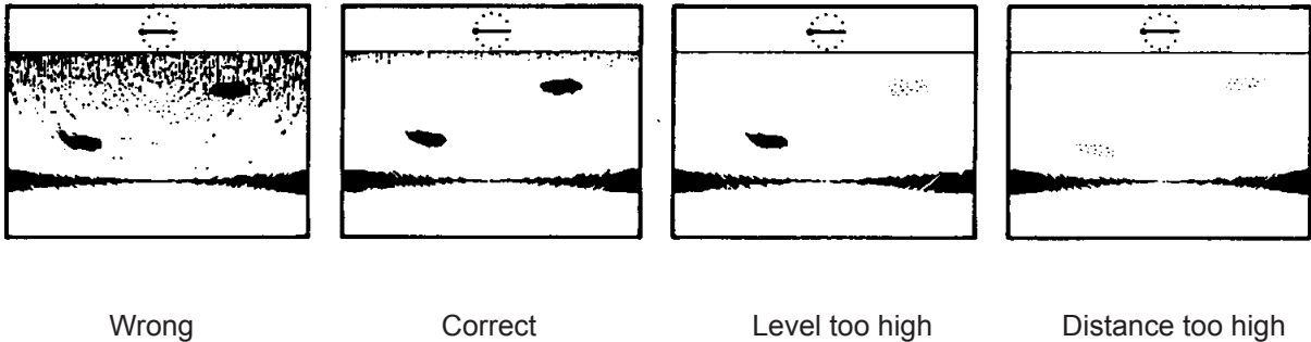
Figure 3-14 Examples of proper and improper TVG
