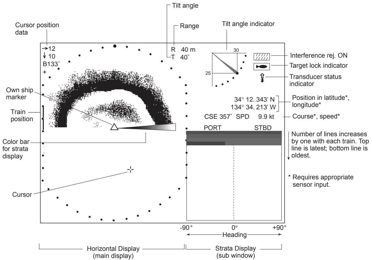
Figure 2-29 Horizontal/strata display
