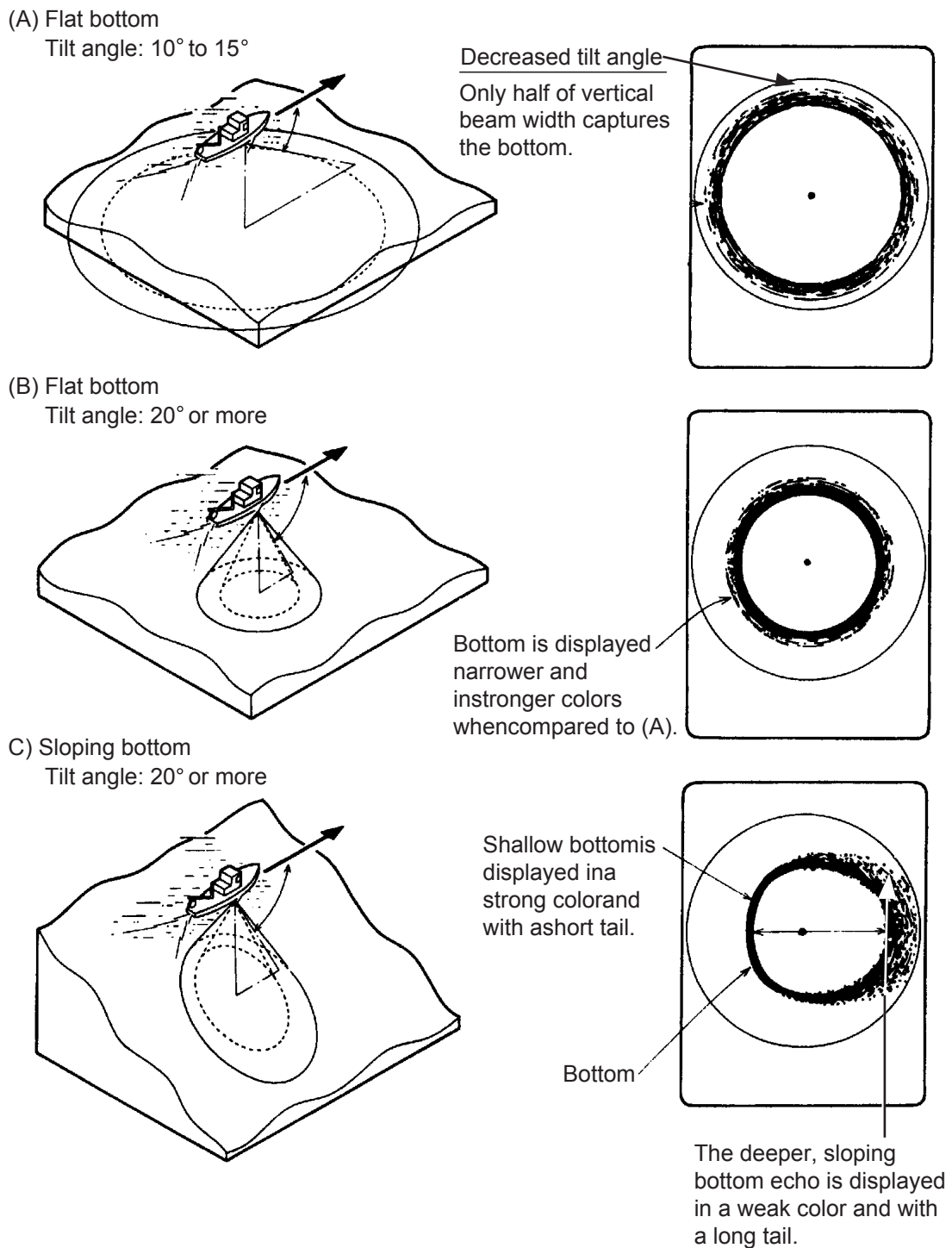
Figure 2-21 Bottom echoes
