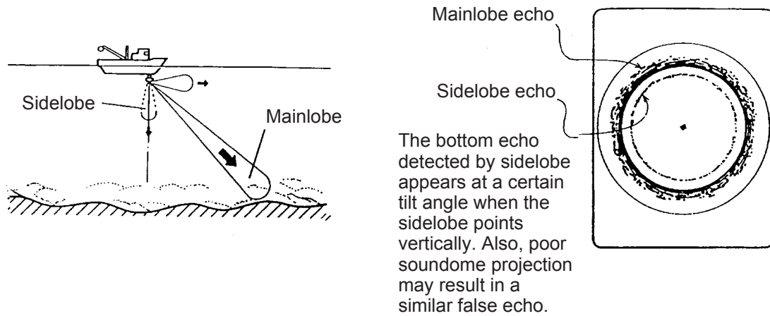
Figure 2-25 Sidelobe echoes
