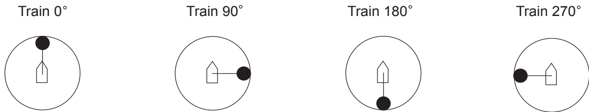
Figure 4-4 Train indicator and display
