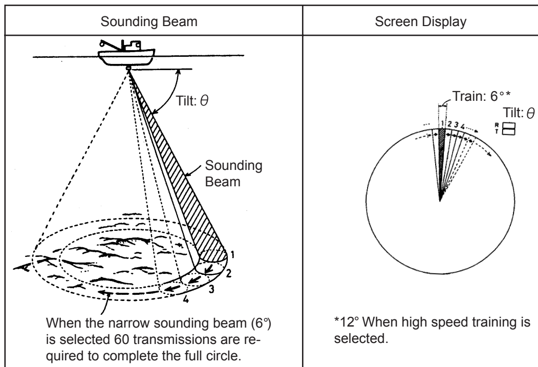
Figure 2-20 How the horizontal mode picture is painted
