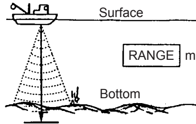
Figure 4-3 Range concept
