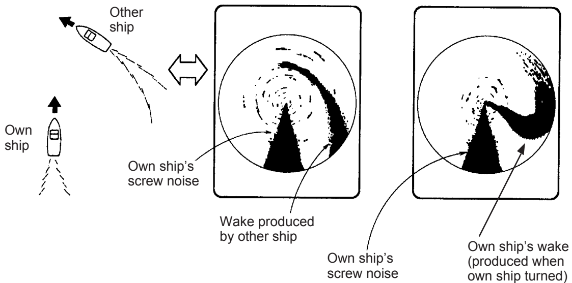
Figure 2-24 Wake
