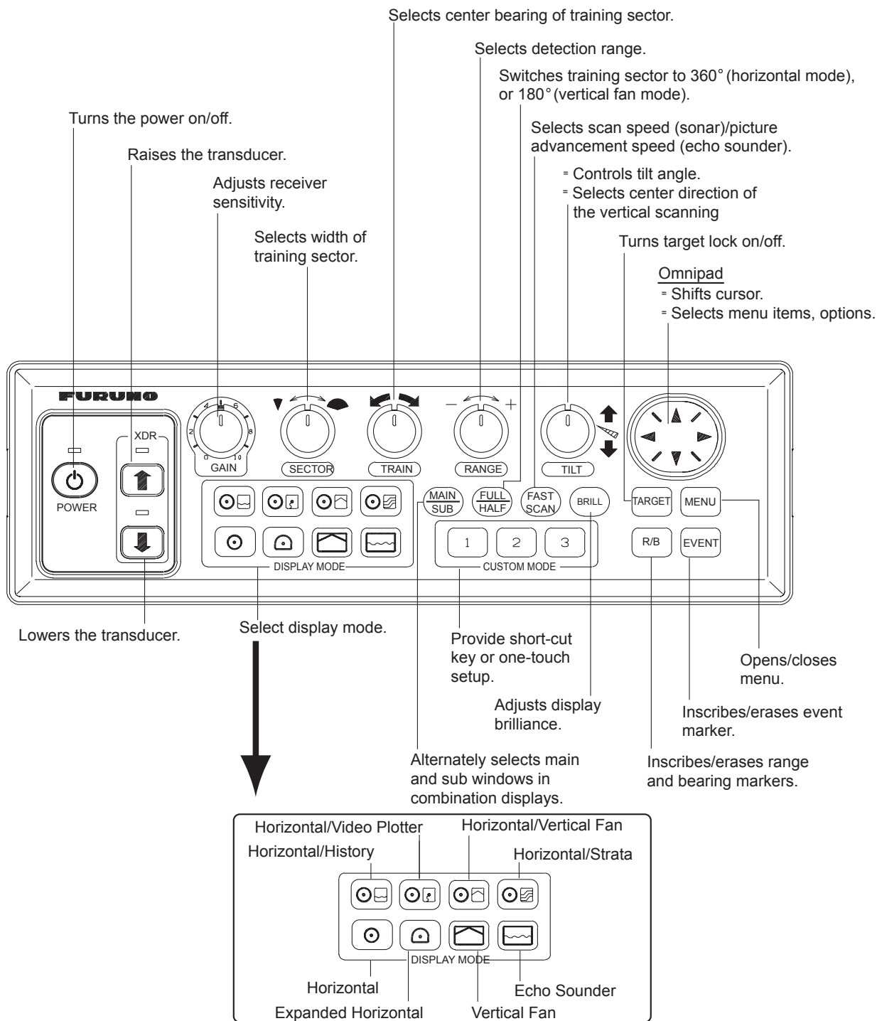
Figure 1-1 Control unit
