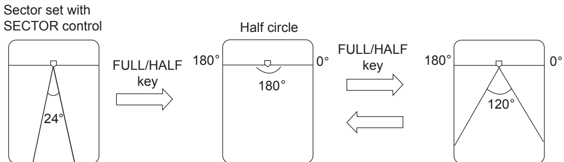
Figure 3-7 How the FULL/HALF key works
