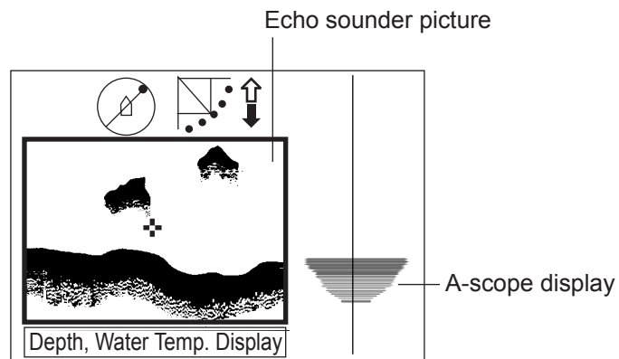
Figure 4-8 A-scope display
