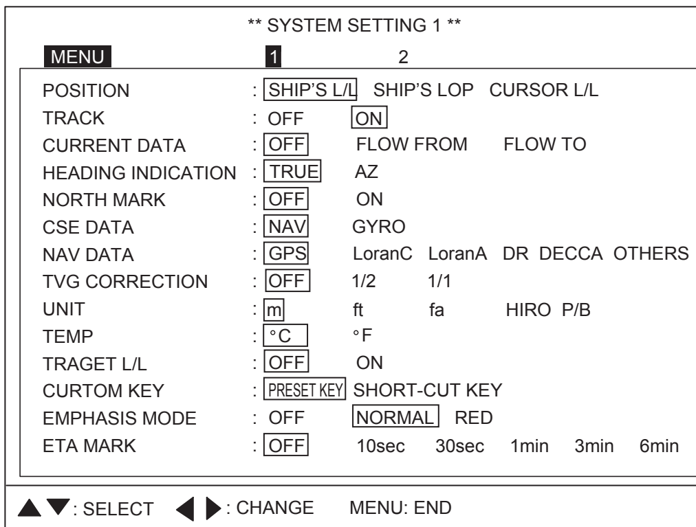
Figure 5-4 System setting 1 menu
