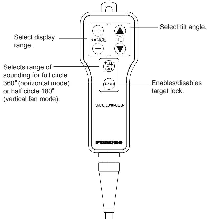
Figure 1-2 Remote controller
