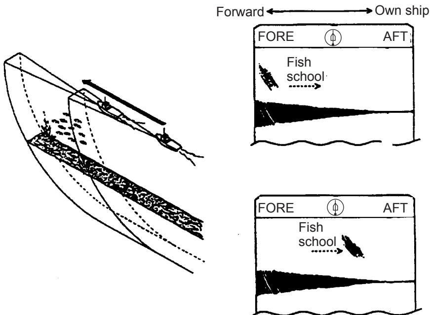
Figure 3-19 Picture appearance when passing over fish schools
