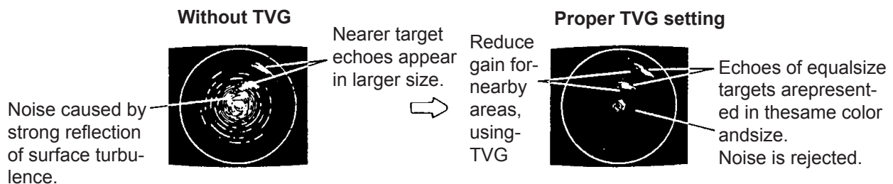
Figure 2-14 How TVG works
