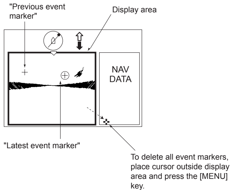
Figure 3-11 How to inscribe, delete the event markers
