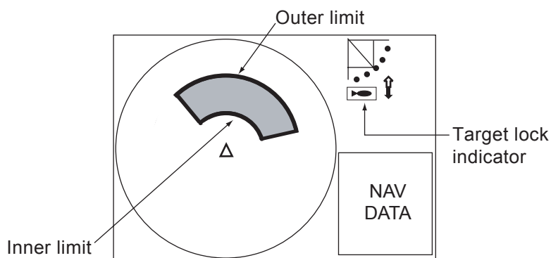
Figure 2-18 Target lock area
