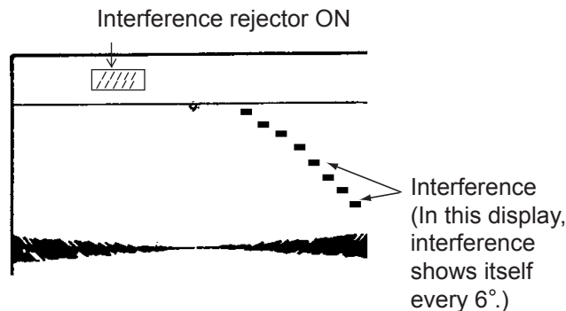
Figure 3-15 Appearance of interference
