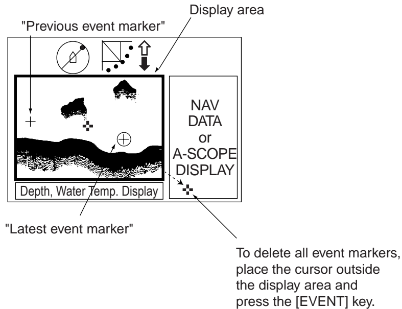
Figure 4-5 How to inscribe, delete the event markers
