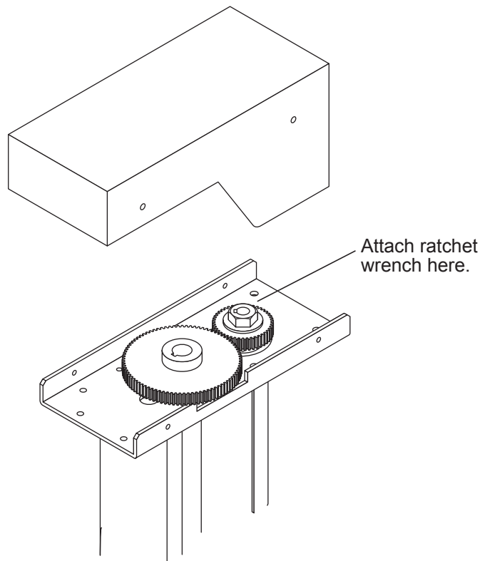
Figure 6-1 Hull unit
