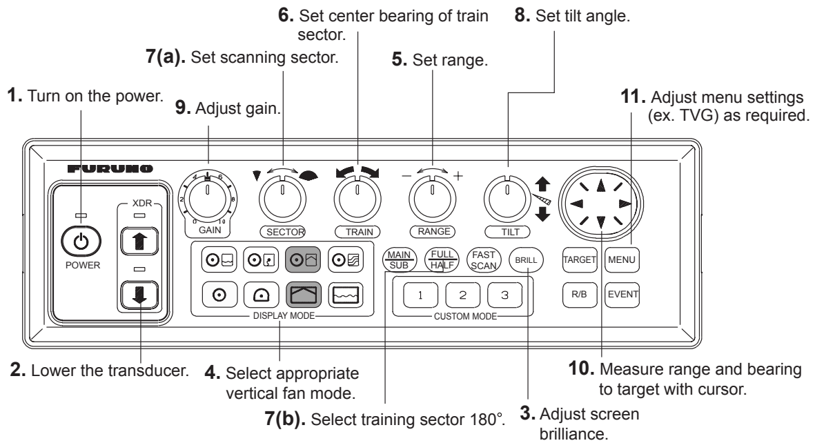
Figure 3-1 Control panel
