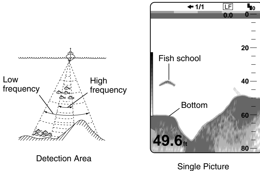
Comparison of detection ranges, sample single picture (low frequency)
