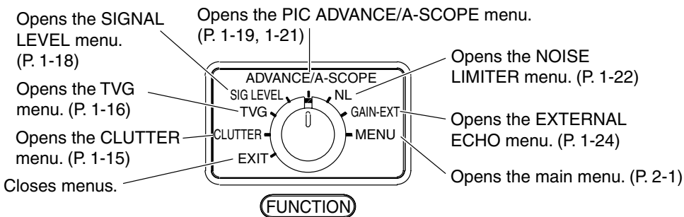
Control unit (Portrait type)
