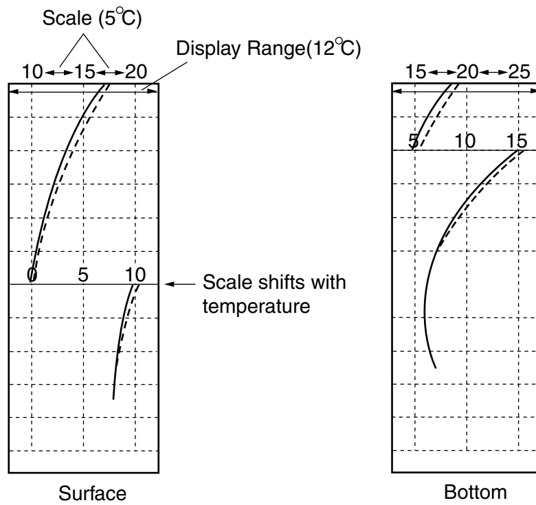
Net sonde water temperature graph (SURFACE/BOTTOM)
