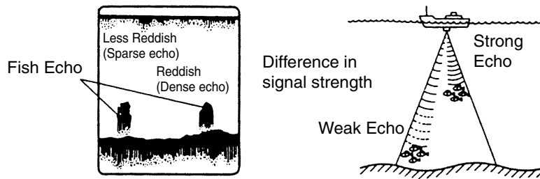
Fish school density
